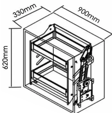
Minimum external cupboard measurements
