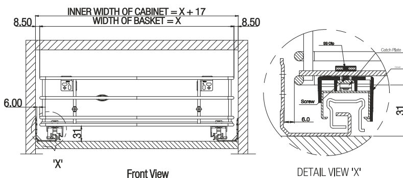
Installation Dimensions with Overlay Facia
